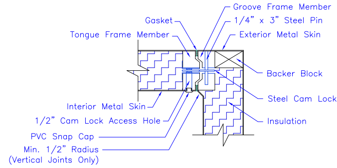
"CAM-LOCK" PANEL CORNER CONNECTION
