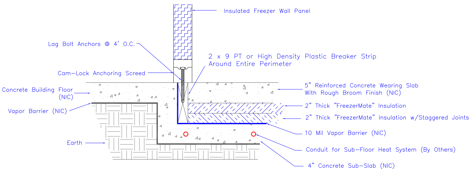
FREEZER SCREED TO BUILDING FLOOR CONNECTION
